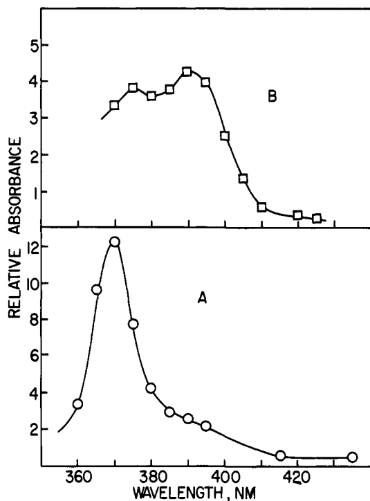
Figure 4. Absorption spectra of radical anion of (A) retinol ( 2.0 \times 10^{-4} M in methanol) observed at 3 \mu\text{s} after the pulse and (B) retinol acetate ( 1.8 \times 10^{-4} M in methanol) observed at 0.2 \mu\text{s} after the pulse.
