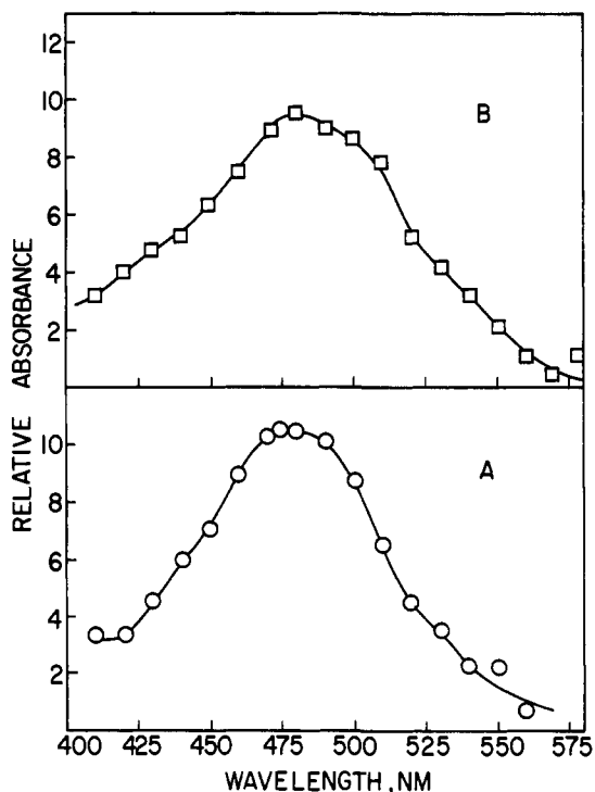
Figure 5. Absorption spectra of radical anion of (A) methyl retinoate ( 1.3 \times 10^{-4} M in methanol) observed at 1.3 \mu\text{s} after the electron pulse and (B) retinoic acid ( 2.0 \times 10^{-4} M in methanol) observed at 0.4 \mu\text{s} after the electron pulse.
