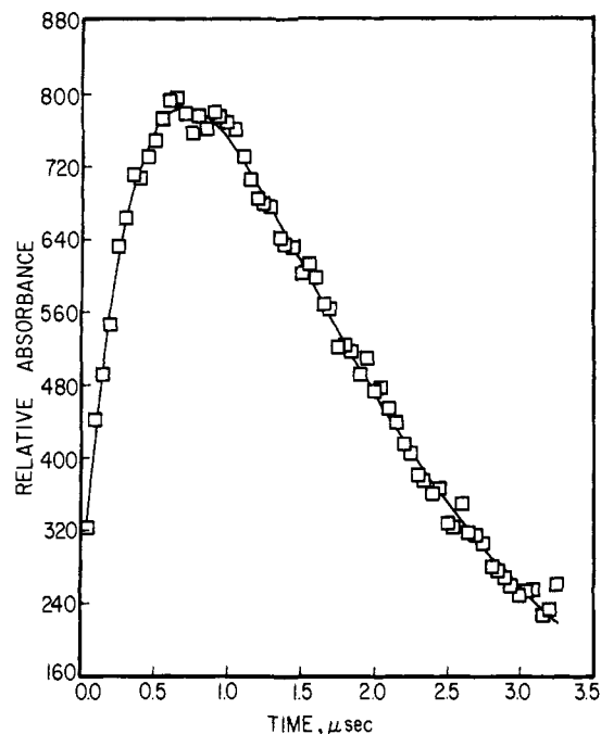
Figure 2. The formation and decay profile for radical anion of methyl retinoate ( 9.0 \times 10^{-5} M in methanol) monitored at 485 nm. The solid line is the least-squares best fit based on two consecutive first-order processes.
