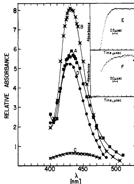
Figure 6. Absorption spectra of transient(s) observed in 2.9 \times 10^{-4} M solution of retinal Schiff base in \text{N}_2 -saturated methanol at (A) 2.0 \mu\text{s} and (B) 350 \mu\text{s} after the pulse, and in \text{N}_2\text{O} -saturated methanol at (C) 1.5 \mu\text{s} and (D) 350 \mu\text{s} after the pulse. Insets: experimental traces showing the formation of radical anion in \text{N}_2 -saturated methanol on (E) short- and (F) long-time scale.
