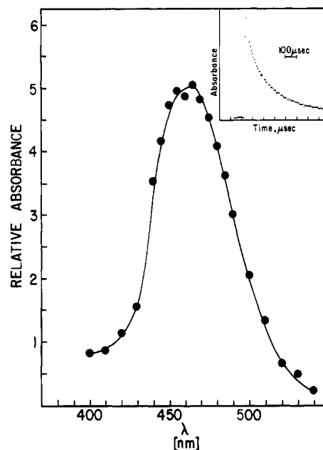
Figure 3. Absorption spectra of radical anion of retinal ( 1.4 \times 10^{-4} M) in 2-propanol, recorded at 2.6 \mu\text{s} following the pulse; inset: experimental trace showing the decay of retinal anion in 2-propanol.
